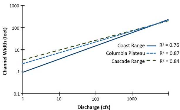
FIGURE 2 Hydraulic geometry relationships for rivers in different Level III Ecoregions in the Pacific Northwest [Colour figure can be viewed at wileyonlinelibrary.com ]
