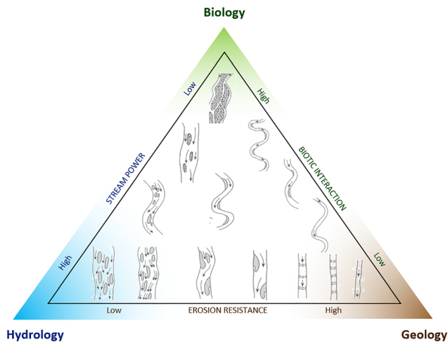
FIGURE 6 The stream evolution triangle (from Castro & Thorne, 2019) [Colour figure can be viewed at wileyonlinelibrary.com ]
