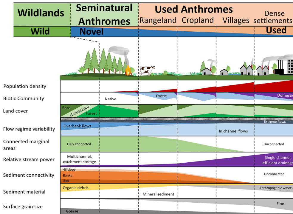
FIGURE 5 Typical stream properties in differing anthromes. Modified from Ellis et al. (2010) [Colour figure can be viewed at wileyonlinelibrary.com ]
